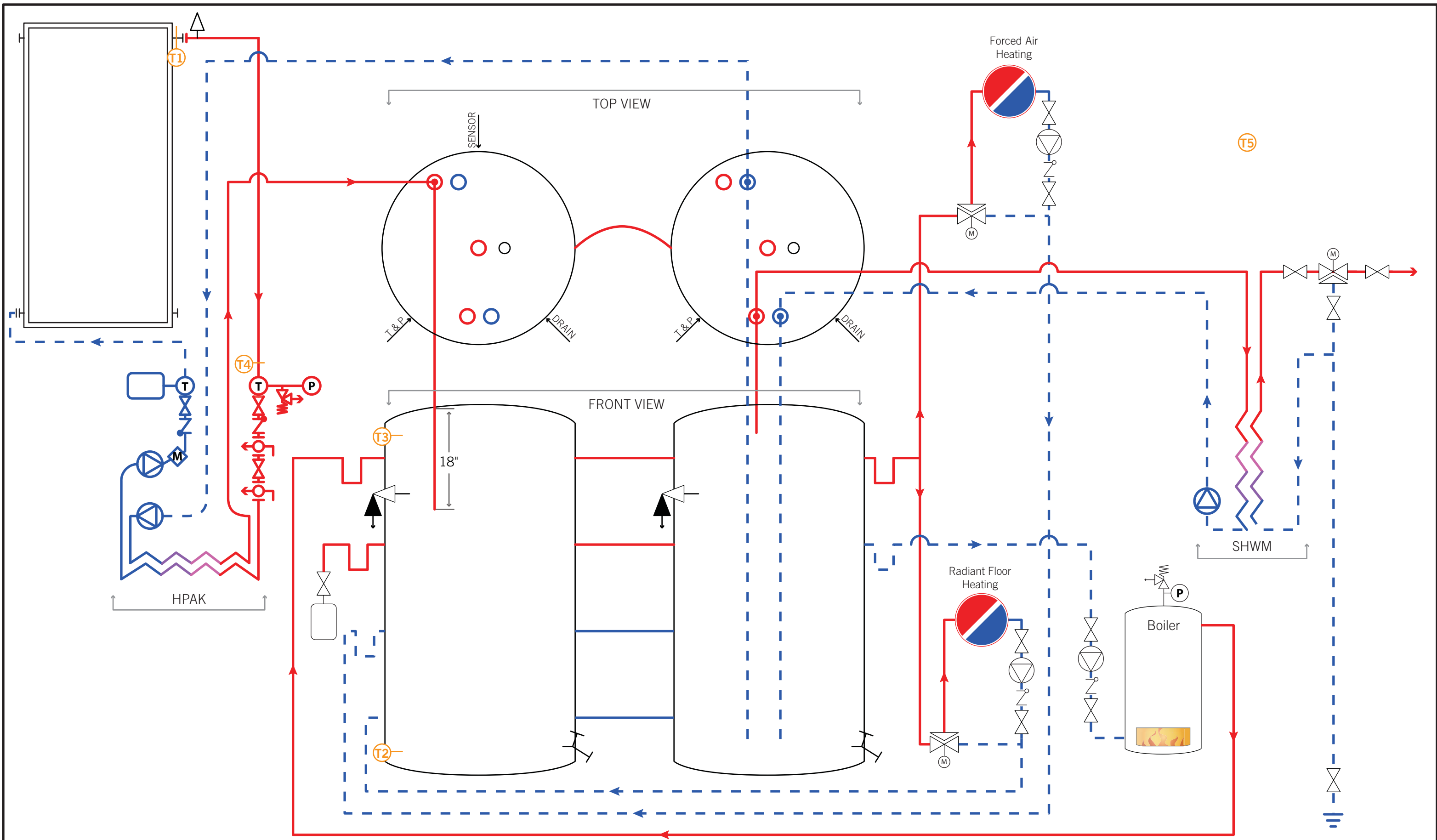
Solar Water and Space Heating Hydraulic Diagram HPAK, Solar Hot Water Module, Helio-Tank 119 with Boiler Backup
