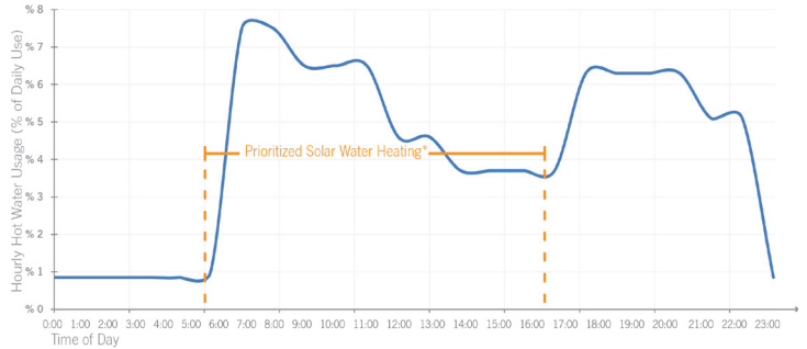
Typical daily hot water usage in an American home
